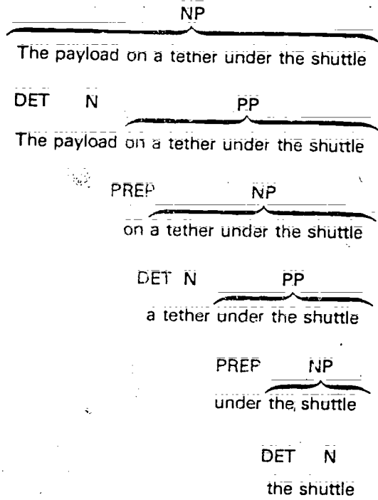
Figure 2. Example Noun Phrase Decomposition.
