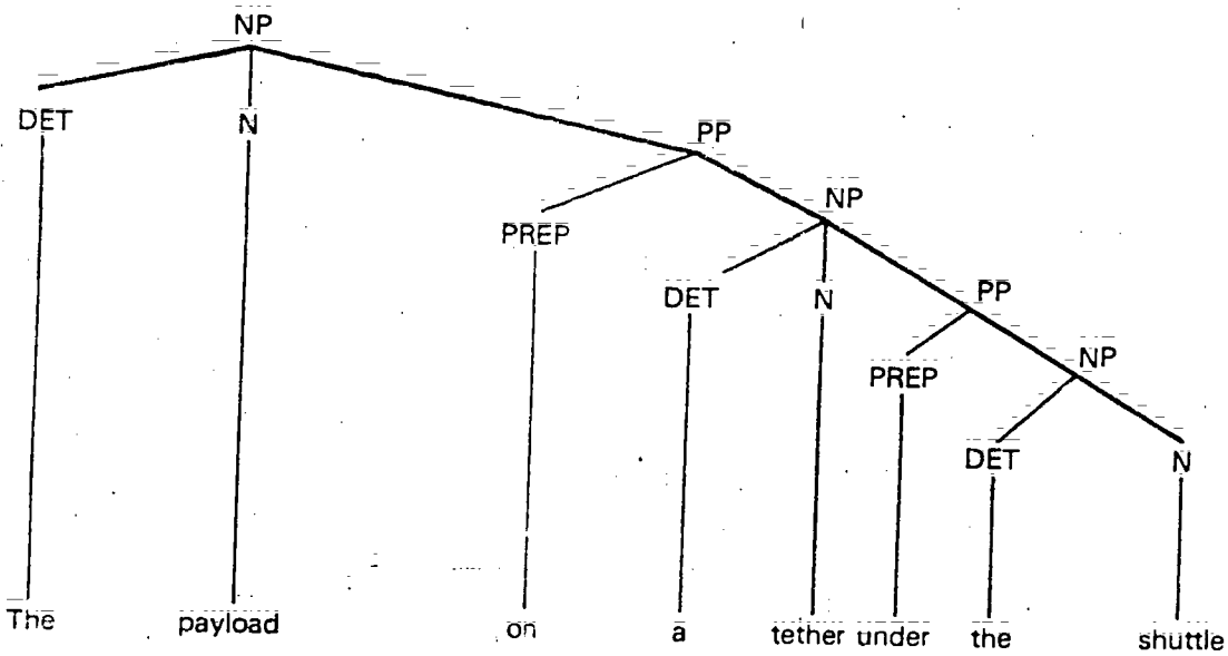
Figure 3. Parse Tree Representation of the Noun Phrase Surface Structure.
